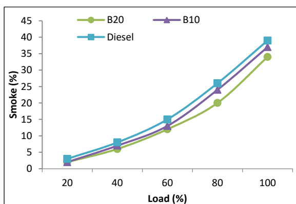
Fig 6: Variation of smoke with load
