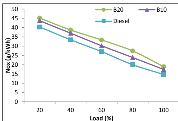
Fig 5: Variation of NOx with Load
